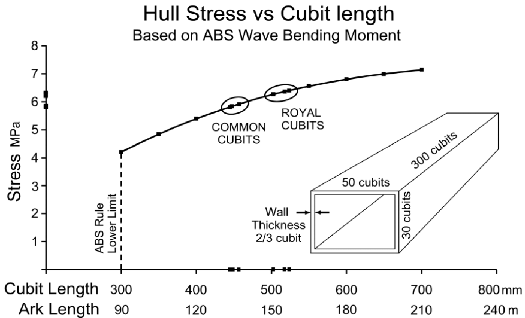
Figure 3. Increase of hull stress with cubit size based on a simple rectangular tube of constant proportions approximating Noah's Ark at various scales. For ships between 90 and 250m long in unrestricted seas, this ABS rule for wave bending moment establishes the hull's necessary bending strength as a function of the vessel's length, breadth and hull form.
